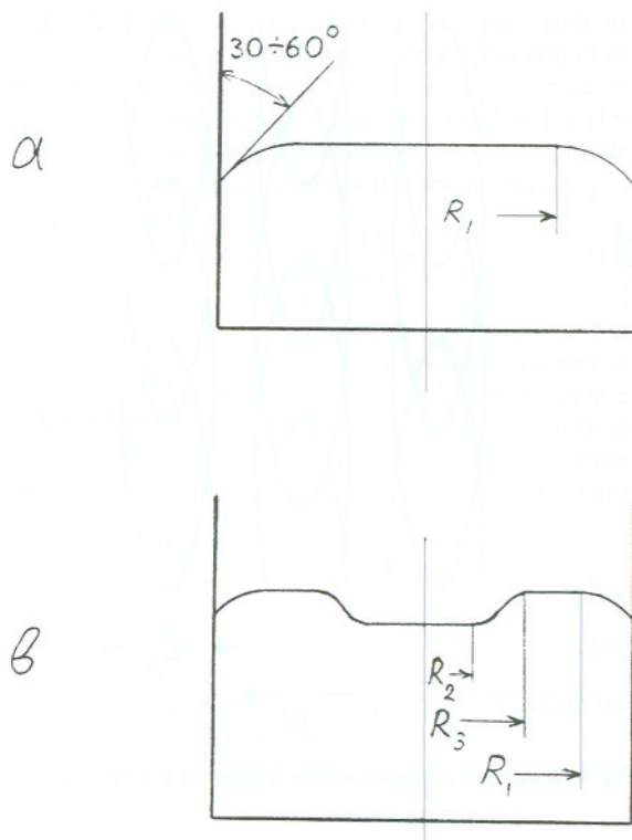
Fig. 5. Splitting of a facet at fast rotation: (a) \Omega < \Omega_c , (b) \Omega > \Omega_c .
